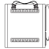
Dometic delibox lite / 444mm x 492mm x 450mm / Max load: 10kg / Fits: All Ösa, All Makka / A food box and backpack in one
